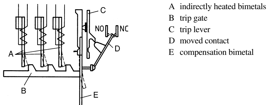
Fig. 6.4.1 Functional principle of a three-pole, thermally delayed thermal relay with temperature compensation. In accordance with IEC, the temperature compensation takes place between -5^{\circ}\text{C} +40^{\circ}\text{C} .
