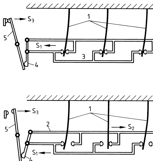
Fig. 6.6.2 Differential tripping principle for thermal relays
