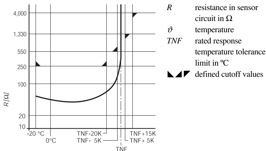
Fig. 5.4.1 Characteristic resistance-temperature curve of a PTC-sensor in line with IEC 34-11-2.
