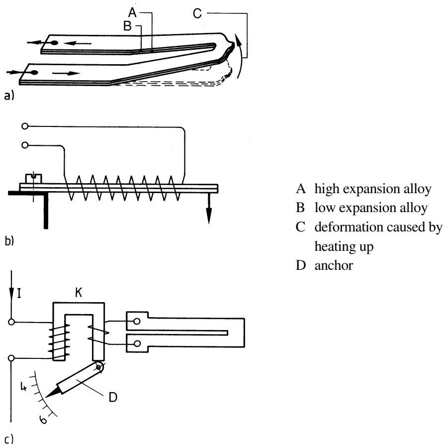
Fig. 6.4.2 Properties of heated bimetals.
