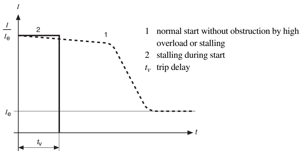
Fig. 6.25.2 Stalling during start.
