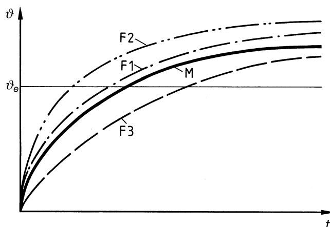
Fig. 6.2.1 Temperature Rise characteristics of a motor and thermal protector for a low overload during continuous operation.
