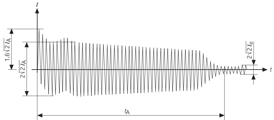
Fig. 2.2.1 Squirrel-cage motor started direct on line (DOL). During starting time t_A , a high motor starting current I_A flows. It does not cause excessive heating if the starting time remains below the limit specified by the motor manufacturer, which is usually 10 sec. The short-term, unbalanced starting current peak can be ignored.
