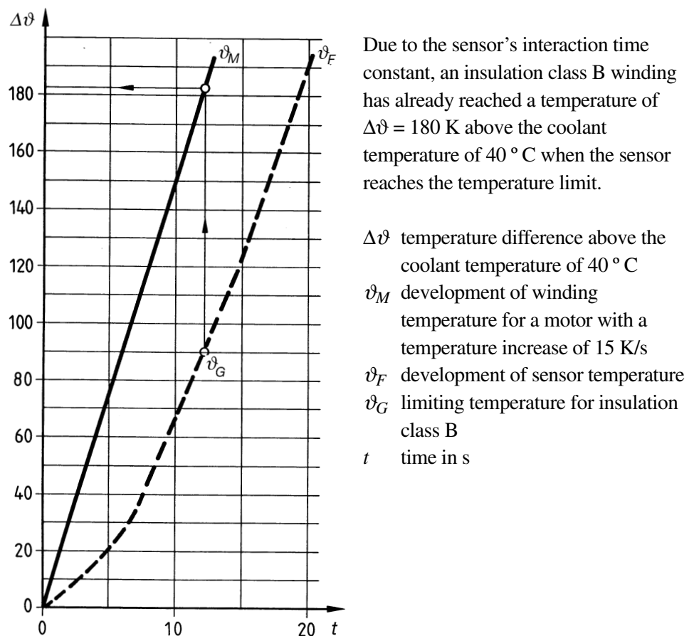
Fig. 5.2.1 Thermal delay of a PTC sensor integrated into the stator winding.
